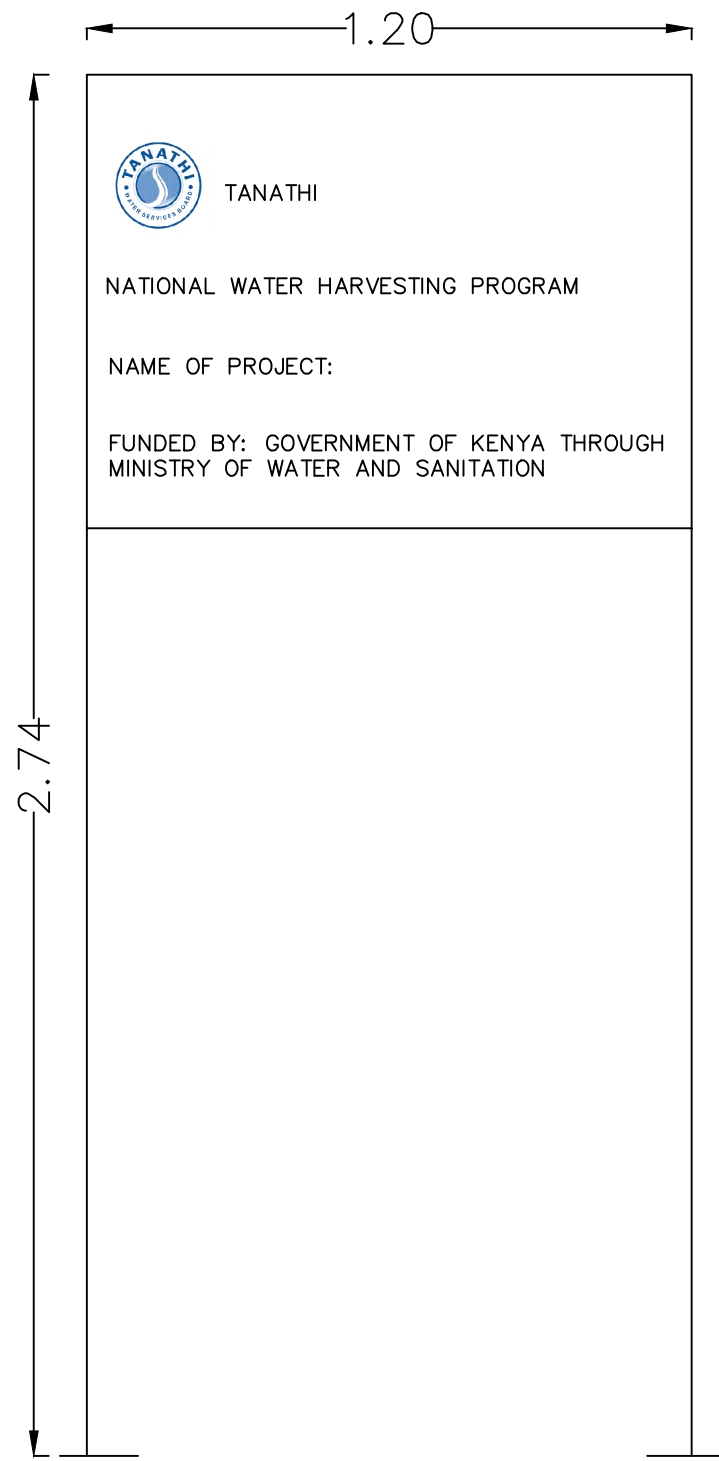
SIGNPOST (Dimensions in metres)
